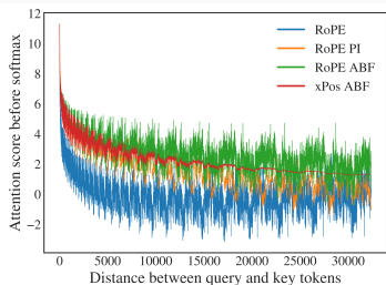
Figure 9: Vanilla RoPE naturally decays as s increases
