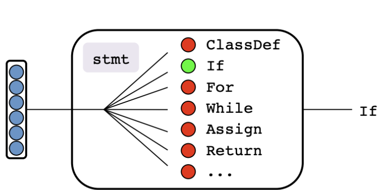
(a) A composite type module choosing a constructor for the corresponding type.
