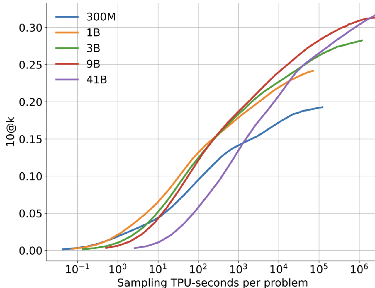
(b) Solve Rate vs. Sampling Compute
